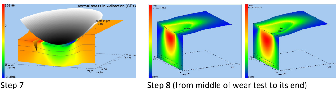
Fig. 9: Practical example for a mechanical surface optimization cycle steps 7 and 8
