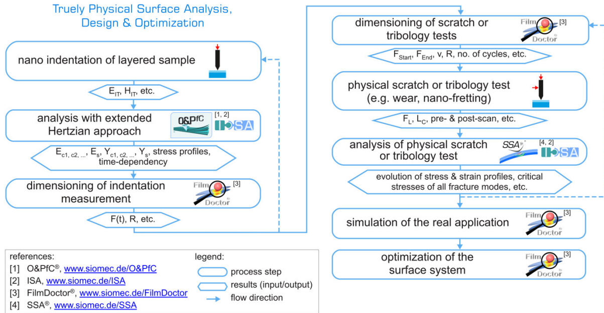
Fig. 1: A flow chart of the procedure of mechanical characterization and optimization of arbitrary structured surfaces with respect to wear and fretting.
