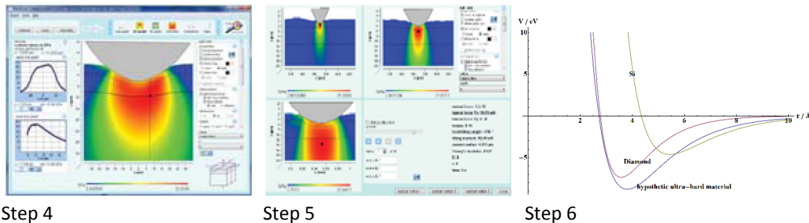
Fig. 8: Practical example for a mechanical surface optimization cycle steps 4 to 6
