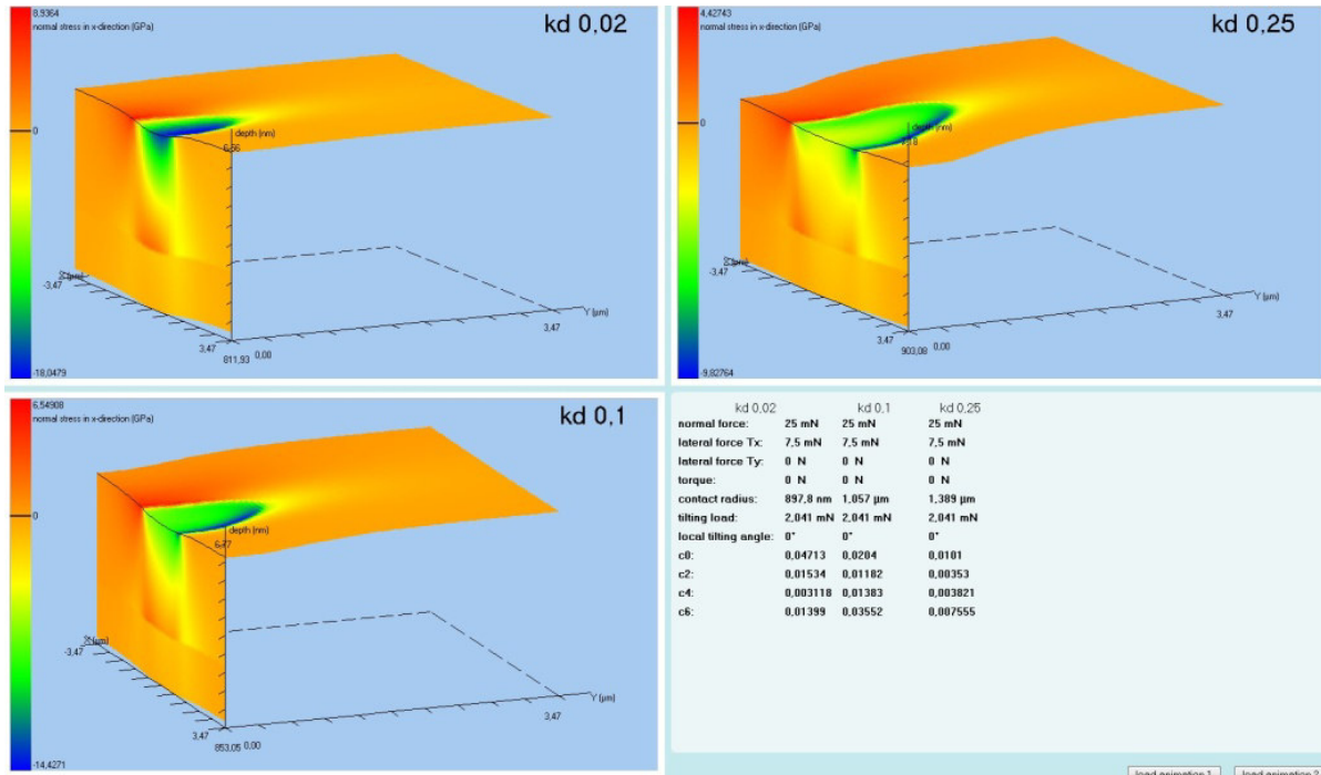
Fig. 19: Wear track evaluation of an oscillating pin (linear wear track) on three different coating materials. End of the Wear test. Normal lateral stress in direction of the moving pin.
