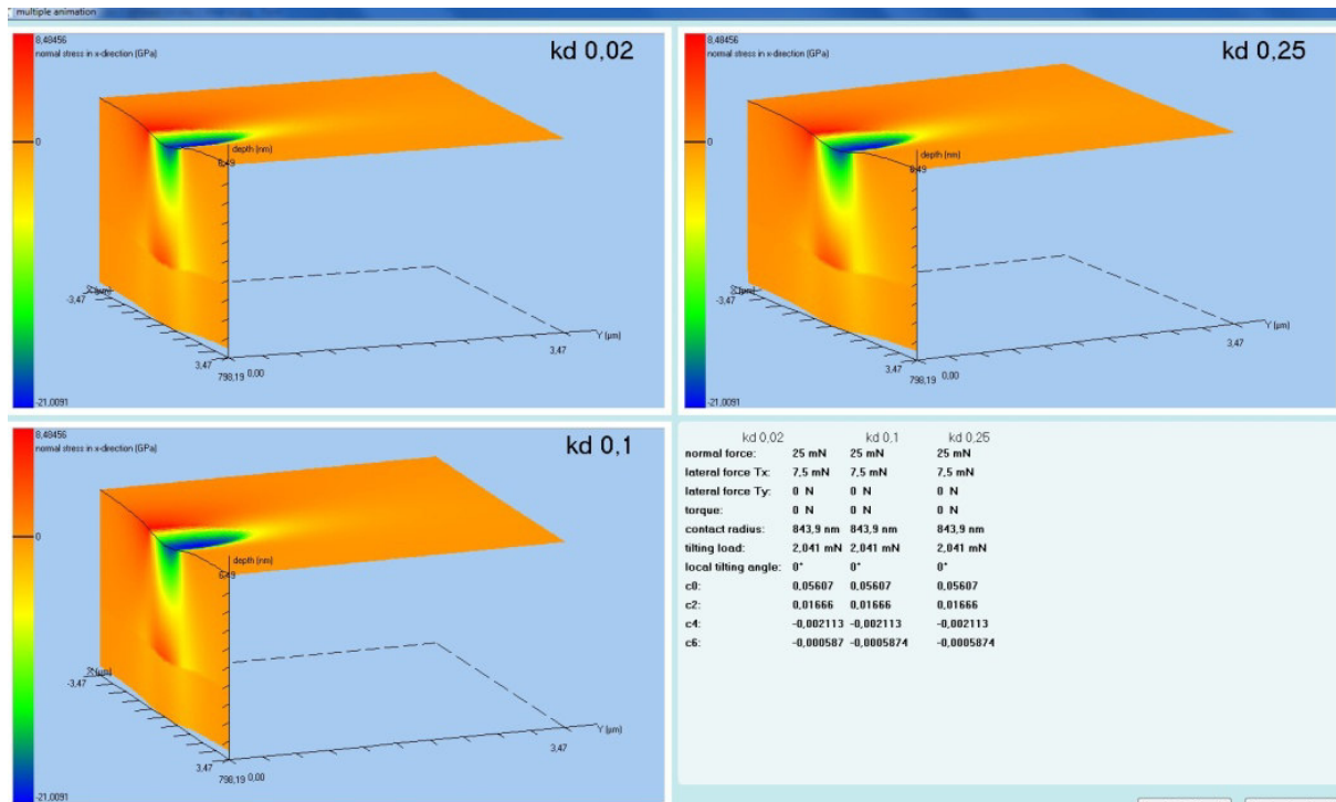
Fig. 13: Wear track evaluation of an oscillating pin (linear wear track) on three different coating materials. Beginning of the Wear test. Normal lateral stress in direction of the moving pin.
