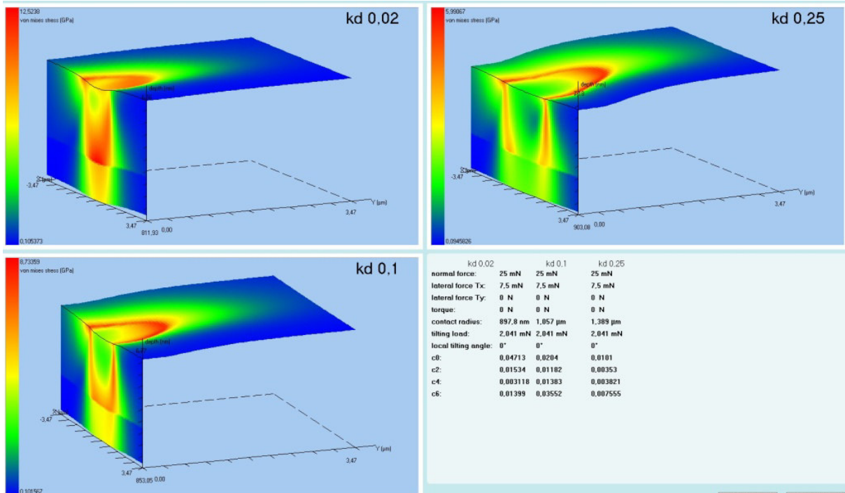
Fig. 17: Wear track evaluation of an oscillating pin (linear wear track) on three different coating materials. End of the Wear test. Von Mises stress.
