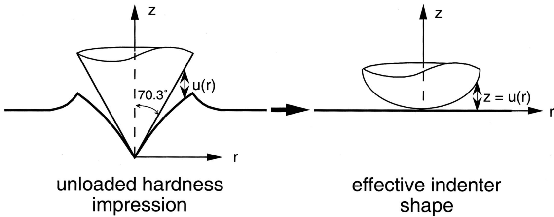
Fig. 2: The effective indenter concept (see: G. M. Pharr, A. Bolshakov: J. Mater. Res., Vol. 17, No. 10, Oct 2002) transferring the theoretically difficult problem of a well defined sharp indenter on an elasto-plastically deformed surface with complex shape (left hand side) to an effective indenter on a flat surface.
