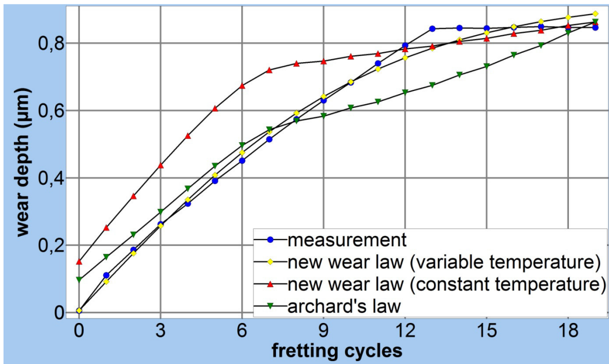
Fig. 21: Comparison of various wear laws with experimental data (c.f. text in section discussion). The data have been reused from [14].
