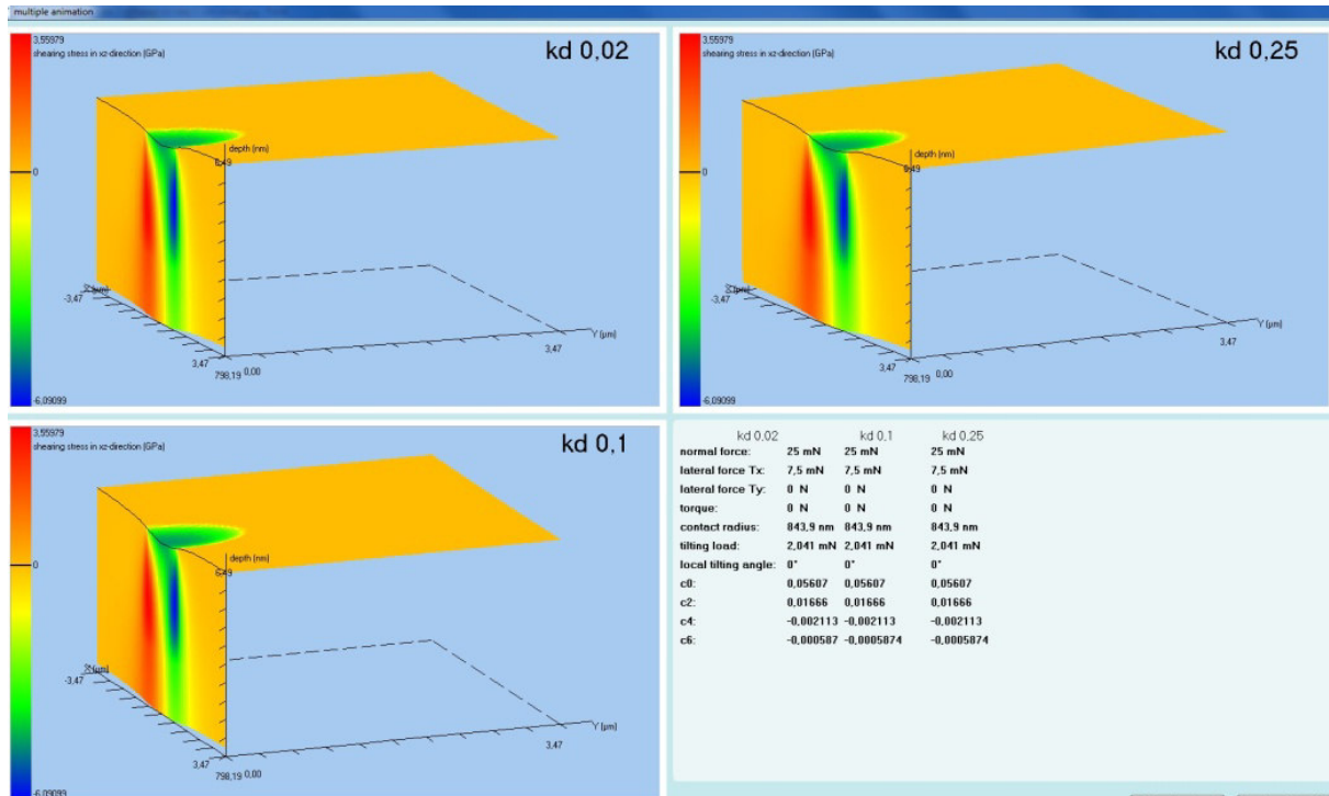
Fig. 12: Wear track evaluation of an oscillating pin (linear wear track) on three different coating materials. Beginning of the Wear test. Shear stress in normal-lateral direction.
