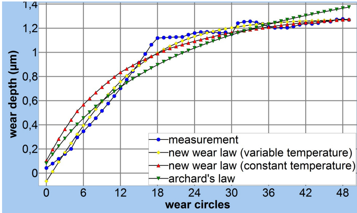
Fig. 20: Comparison of various wear laws with experimental data (c.f. text in section discussion). The data have been reused from [13].
