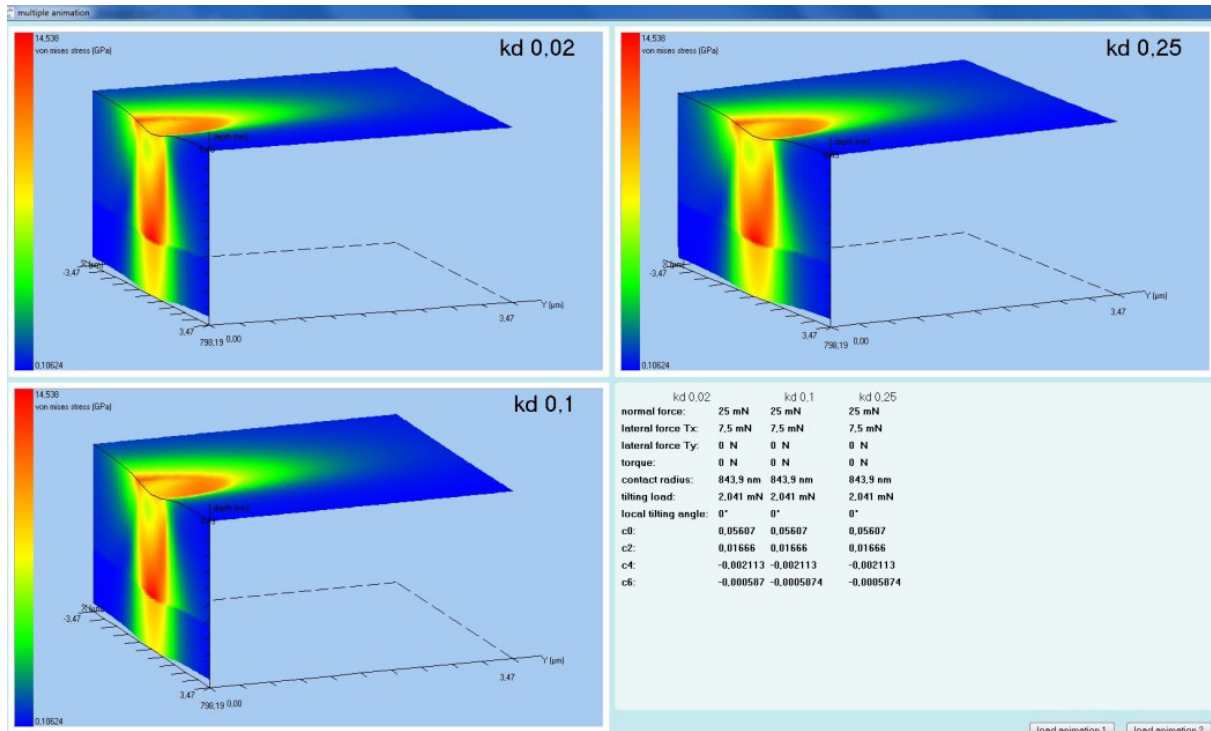
Fig. 11: Wear track evaluation of an oscillating pin (linear wear track) on three different coating materials. Beginning of the Wear test. Von Mises stress.
