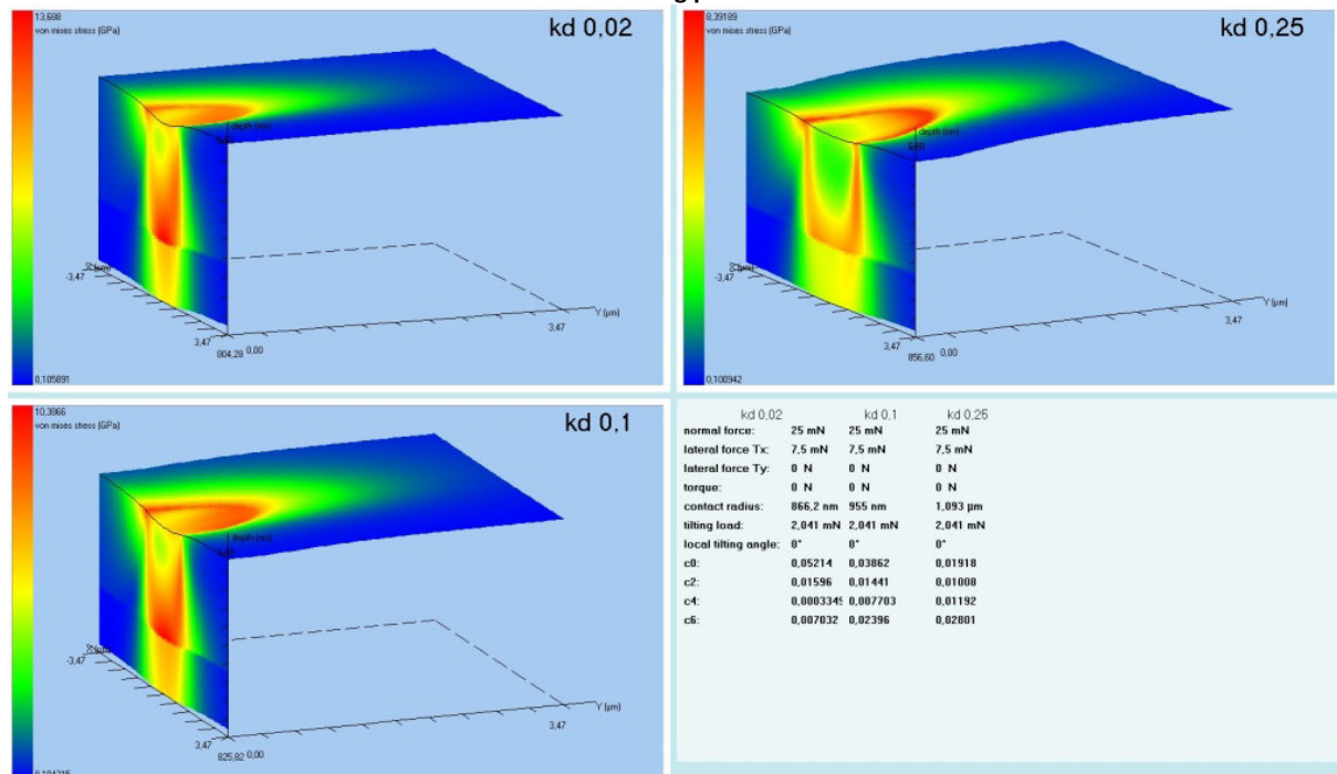
Fig. 14: Wear track evaluation of an oscillating pin (linear wear track) on three different coating materials. Middle of the Wear test. Von Mises stress.
