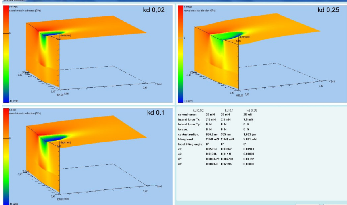
Fig. 16: Wear track evaluation of an oscillating pin (linear wear track) on three different coating materials. Middle Beginning of the Wear test. Normal lateral stress in direction of the moving pin.
