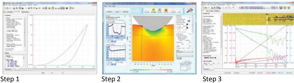
Fig. 7: Practical example for a mechanical surface optimization cycle steps 1 to 3
