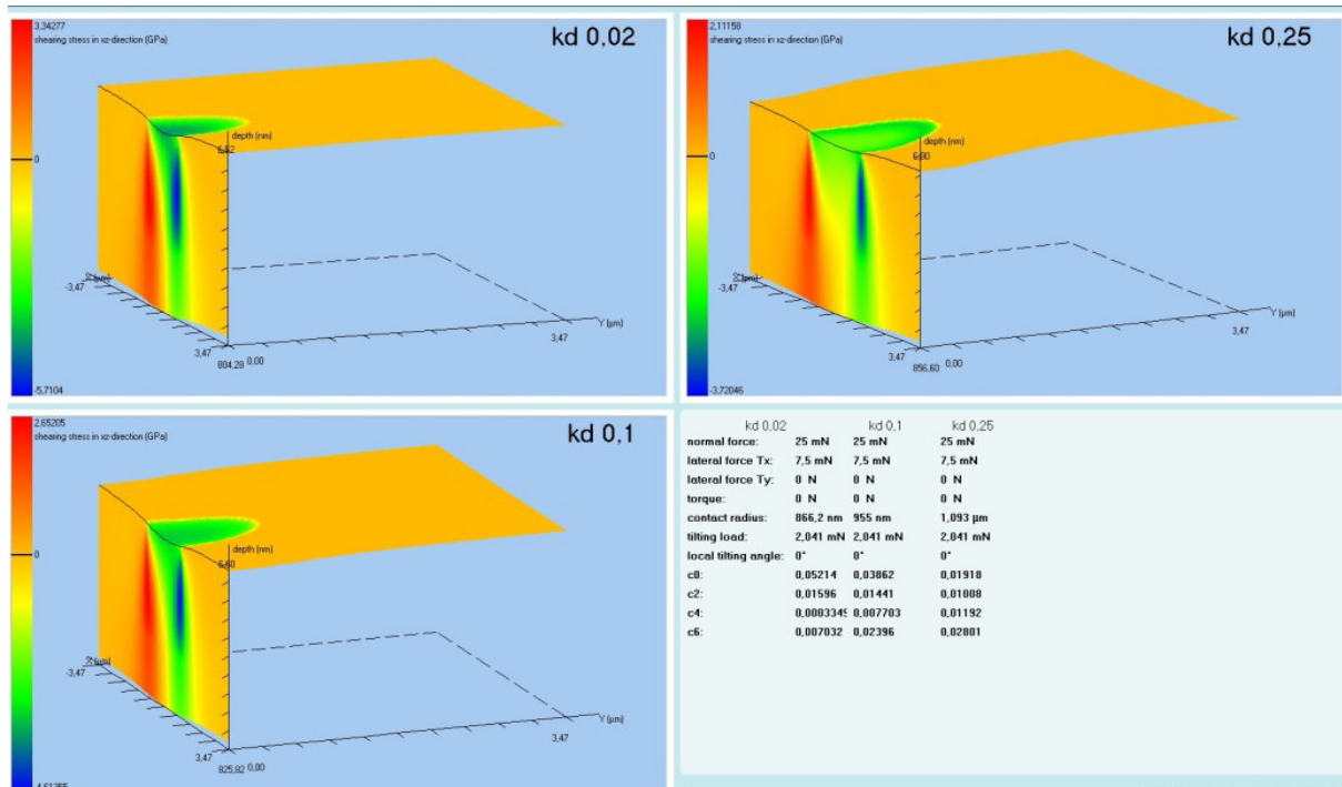
Fig. 15: Wear track evaluation of an oscillating pin (linear wear track) on three different coating materials. Middle of the Wear test. Shear stress in normal-lateral direction.
