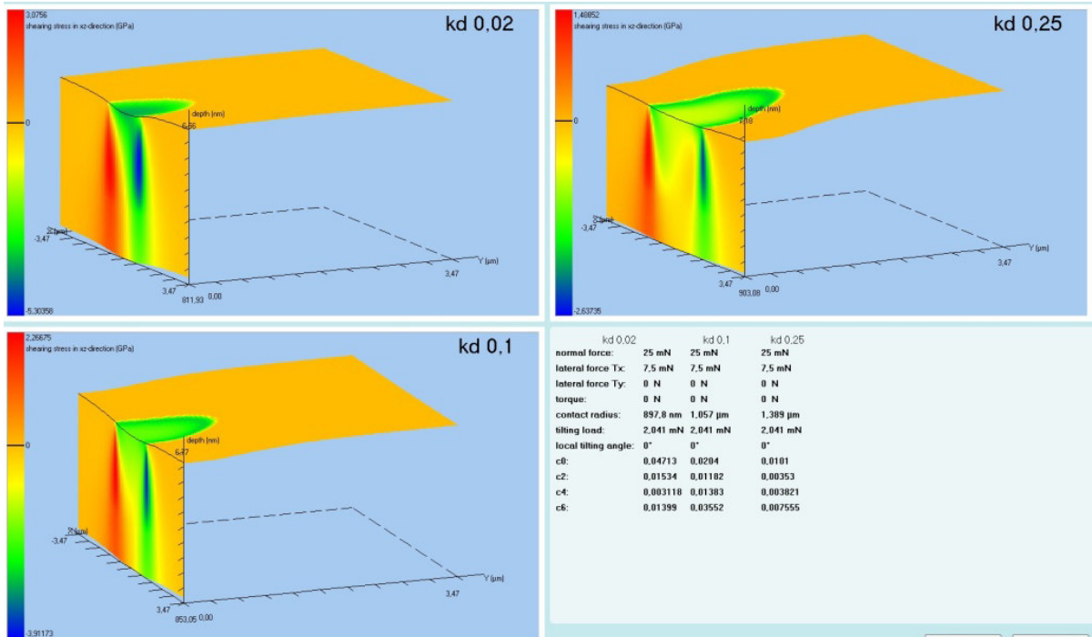
Fig. 18: Wear track evaluation of an oscillating pin (linear wear track) on three different coating materials. End of the Wear test. Shear stress in normal-lateral direction.
