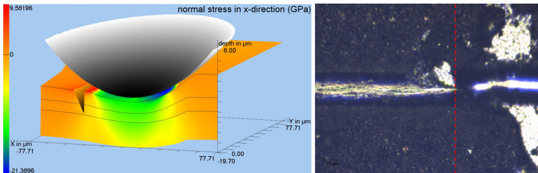
Fig. 6: Illustrative scheme of the failure mechanism (a) and an optical graph of the post-scratch surface (b) in which the corresponding L_c position is marked by the red dashed line (from [12]).
